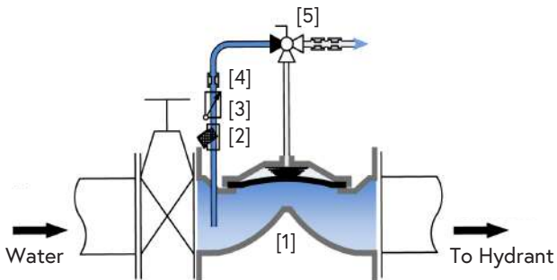
Manually Actuated
