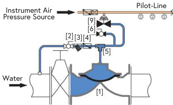
Standby Position
