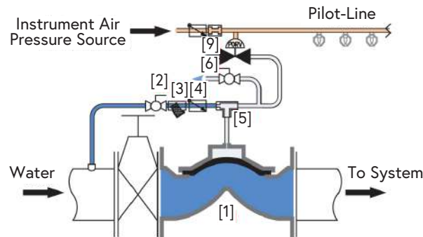
Manually Actuated
