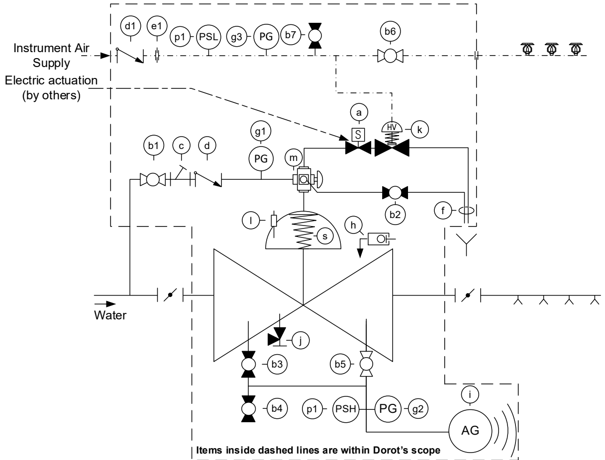
Fig. 2- System P&ID
