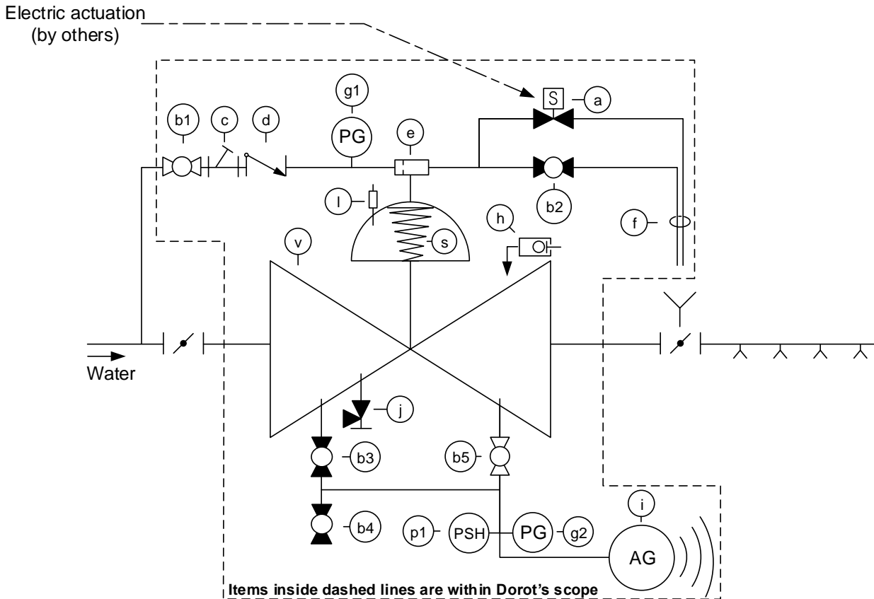
Fig. 2- System P&ID
