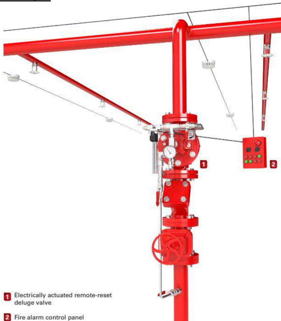
Fig. 1- General layout
