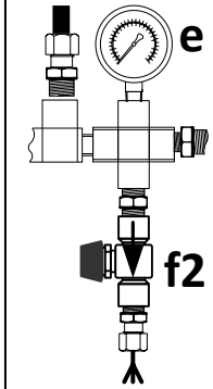
Drawing 3 L.P Simulation Trim
